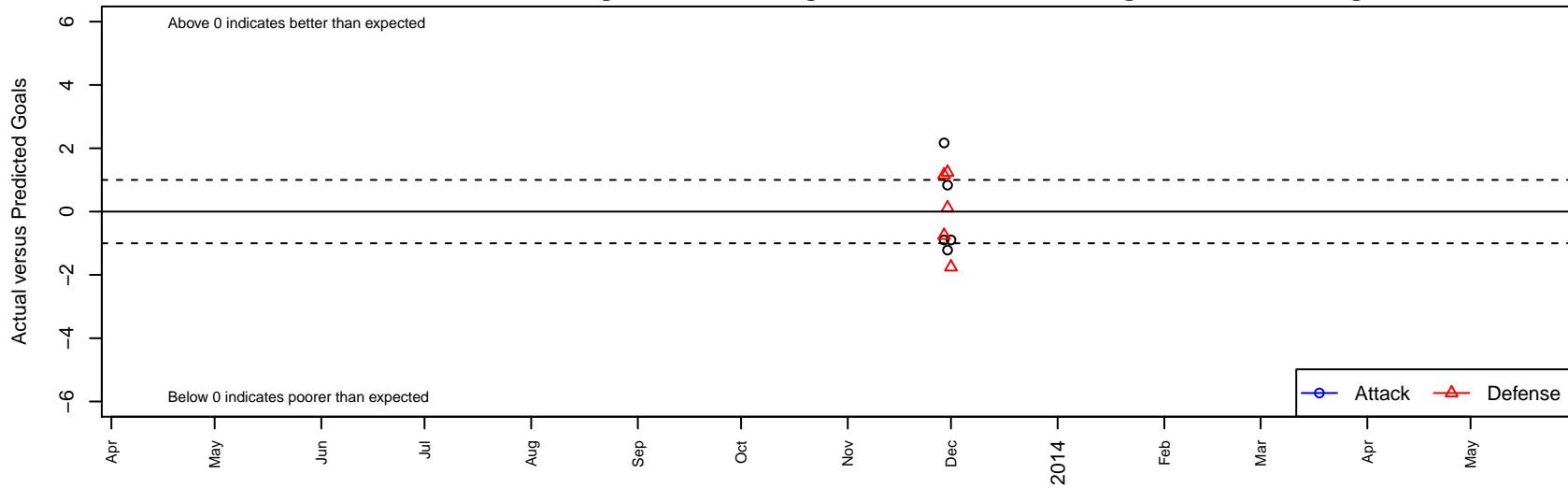
Xolos Academy Red B01 Dots are actual minus expected GF (blue circles) and GA (red triangles). Blue line is smoothed change in attack strength. Red is smoothed change in defense strength.
